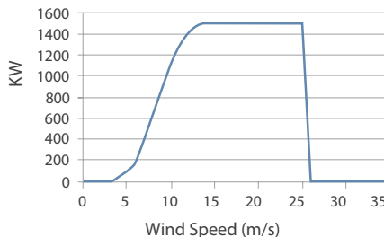
Power Curve
