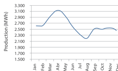
Power Production
